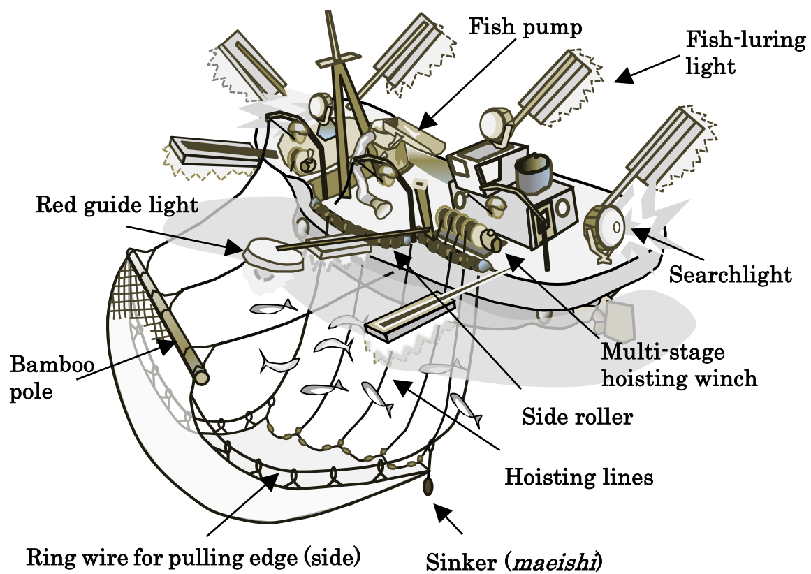
Figure 39 Illustration of stick-held dip net fishing operations
