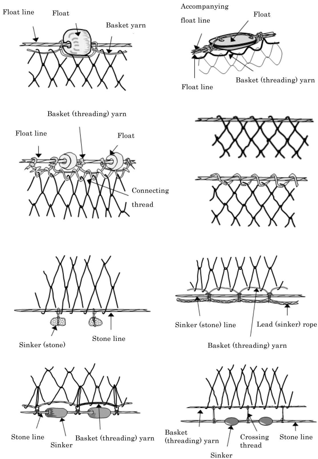
Figure 21: Various sewing methods of float part and sinker part
