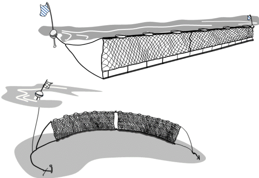
Figure 17: Surface layer flowing type (top figure) and bottom layer fixed type (bottom figure) gill nets
