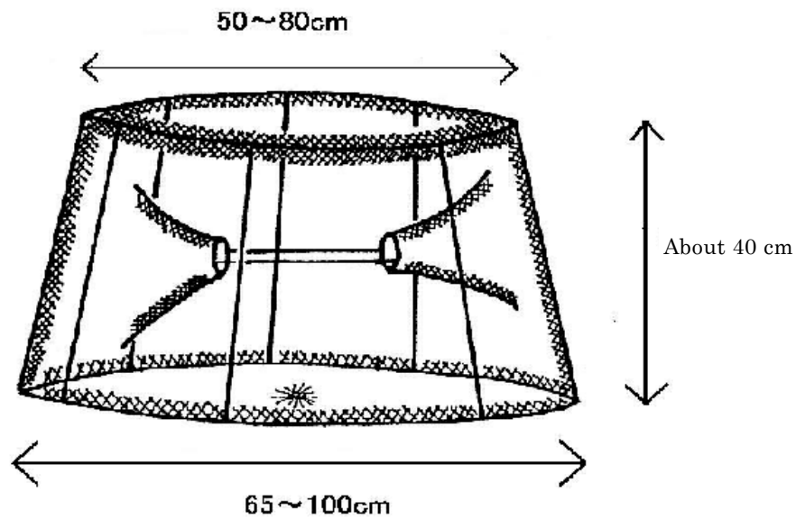
Figure 36: Shape of a shrimp basket
