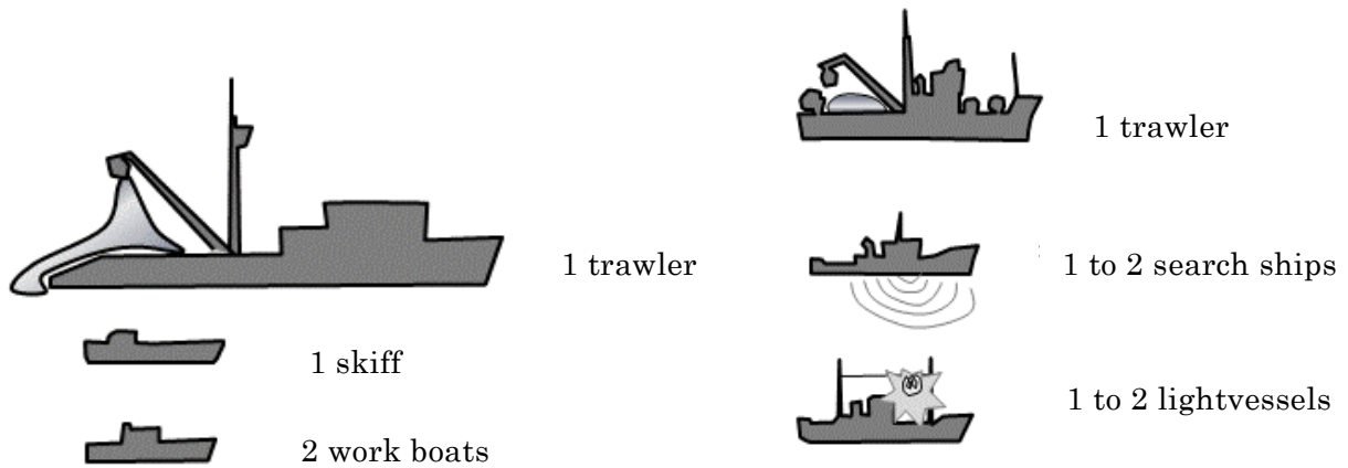
Figure 1: Single-ship roundhaul system structure (the skiff and work boats are loaded on the trawler)
