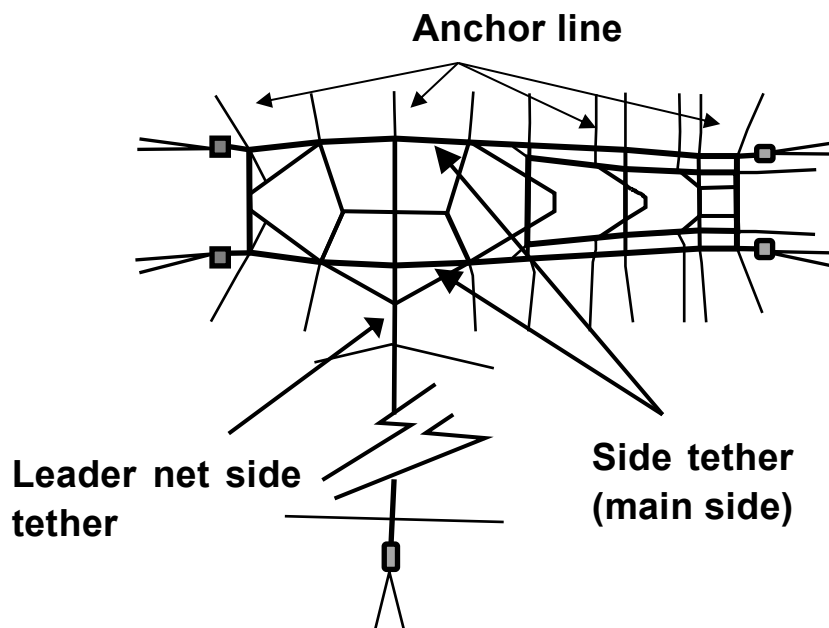
Figure 28: Side tethers of a fixed net
