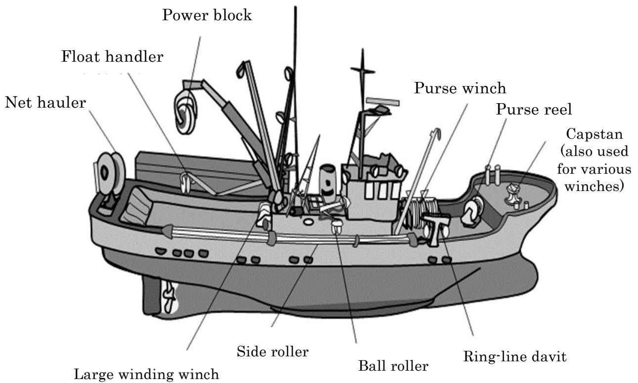
Figure 3-1: Fishing devices on trawler
