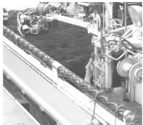
Figure 5: Side roller
