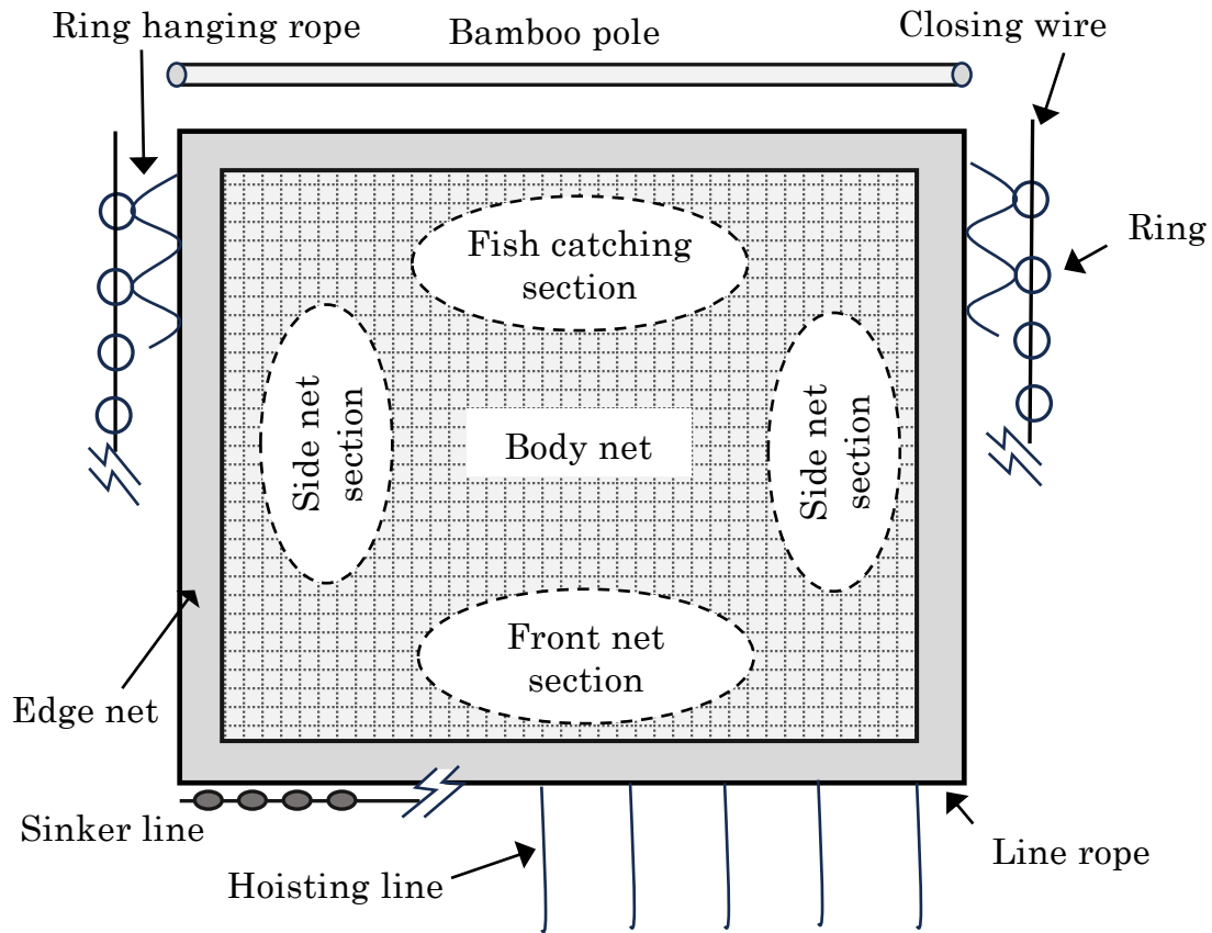
Figure 40: Schematic diagram of stick-held dip net
