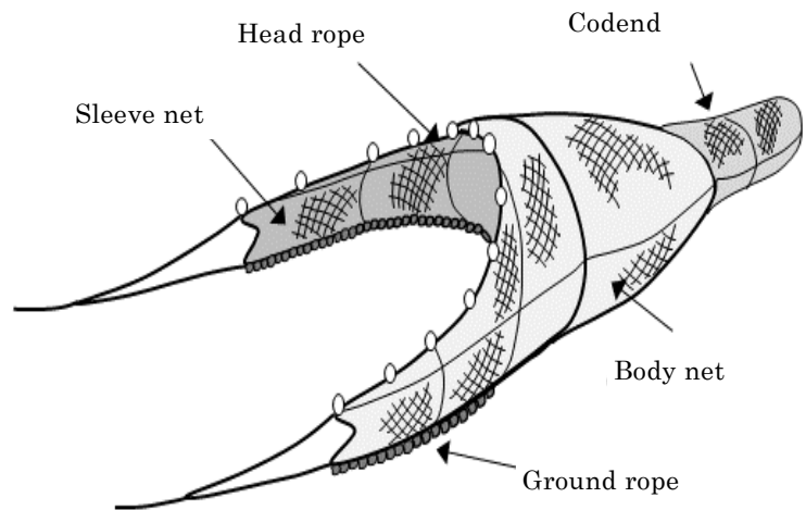
Figure 22: Names of major parts of trawl nets
