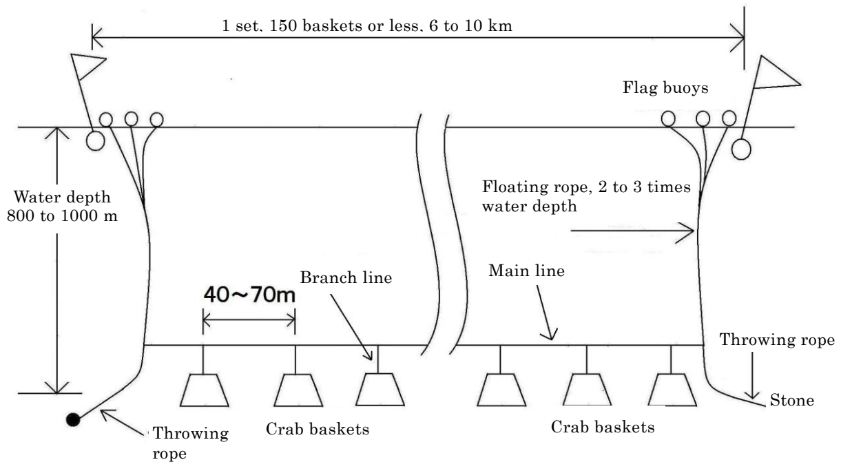
Figure 34: Arrangement of fishing tool installations
