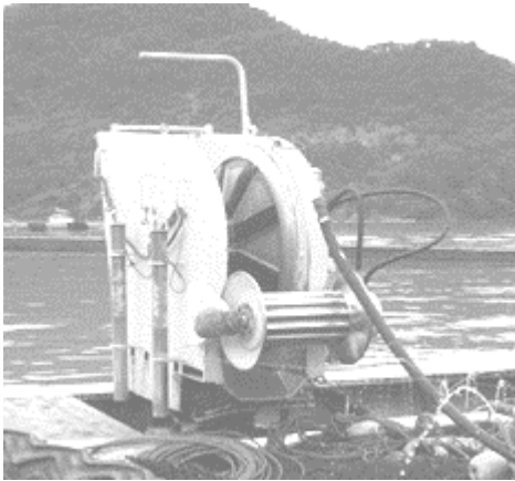
Figure 4-1: Net hauler
