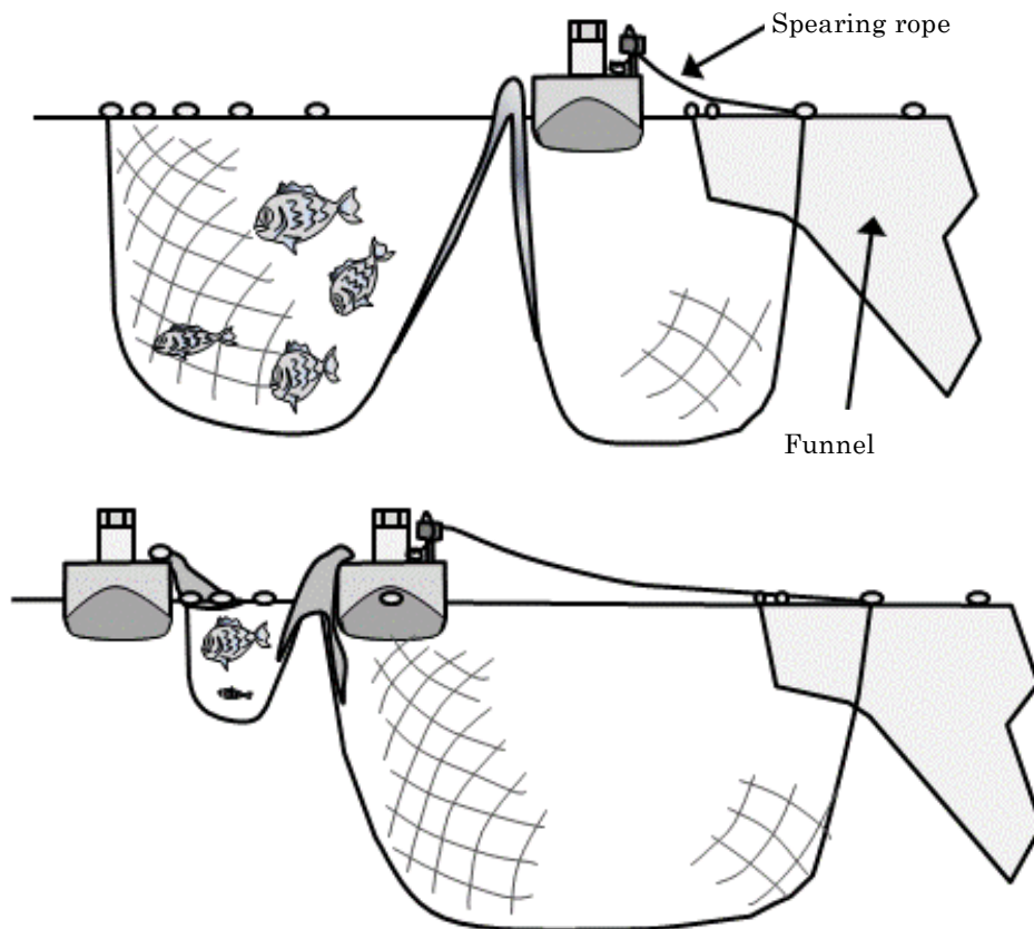
Figure 31: A cross-sectional view of net hauling work The top figure is B from Figure 30, and the bottom figure indicates the state of C.
