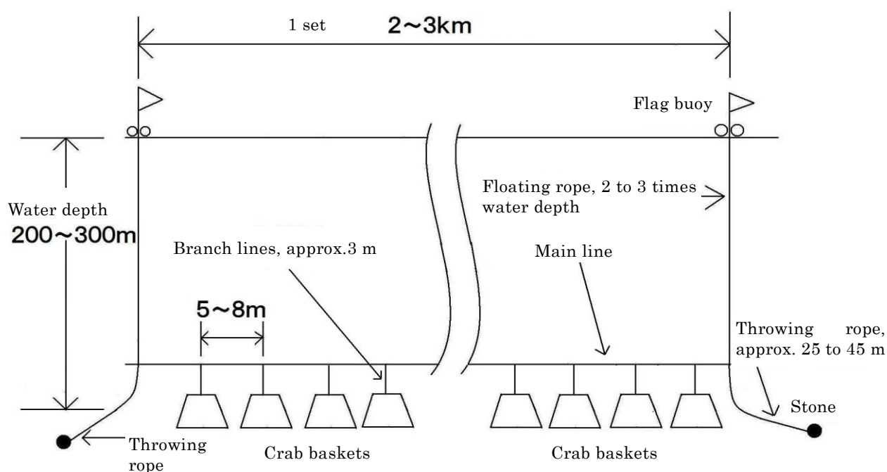
Figure 37: Conditions when shrimp baskets have been cast into the sea
