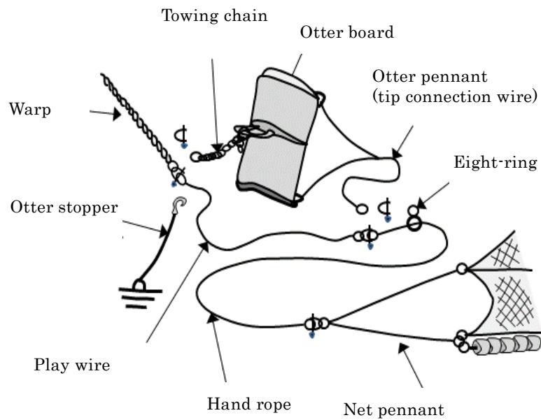
Figure 24: Otter trawl rigging
