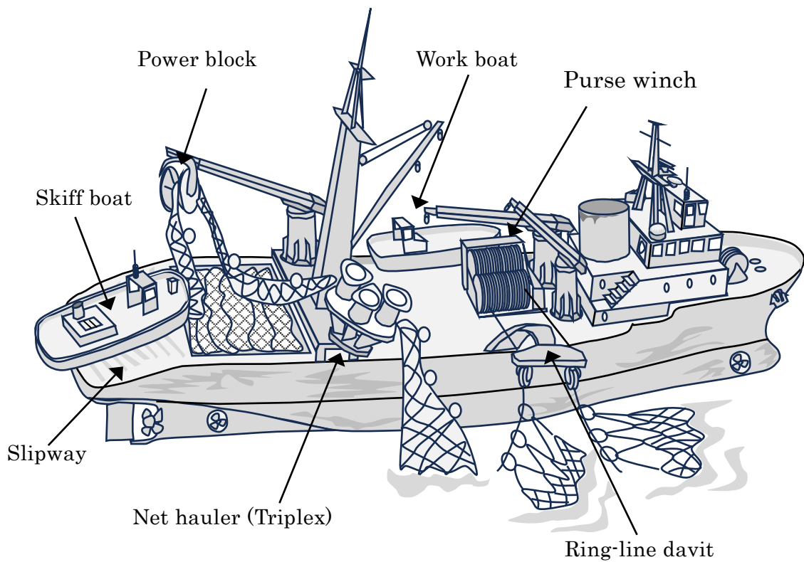
Figure 3-2: Trawler in recent years
