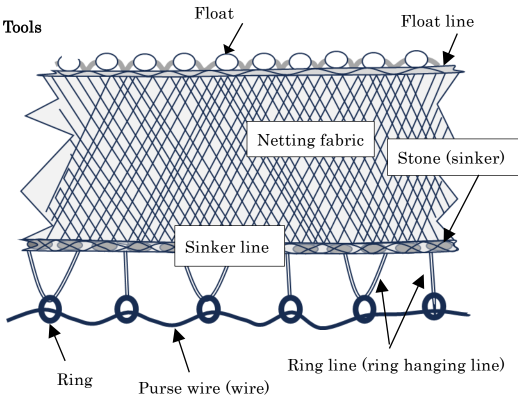
Figure 12: Roundhaul net structure and names of parts
