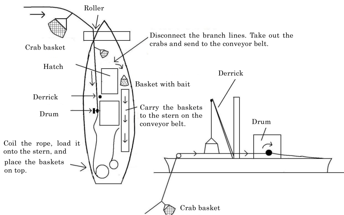
Figure 35: Main elements of basket hoisting operations for red snow crab basket fishing
