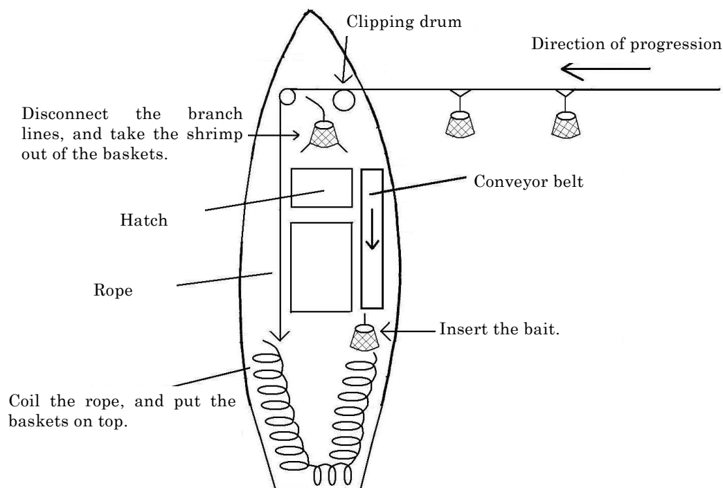
Figure 38: Shrimp basket fishing hoisting method
