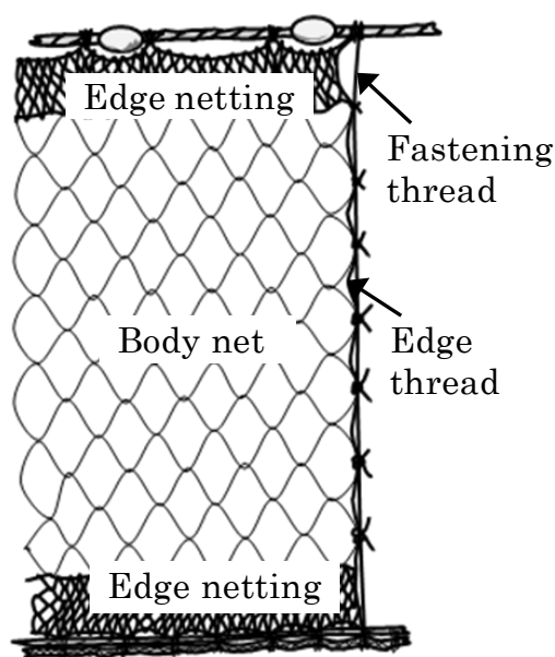
Figure 20: Edge sewing (net) and edge fastening
