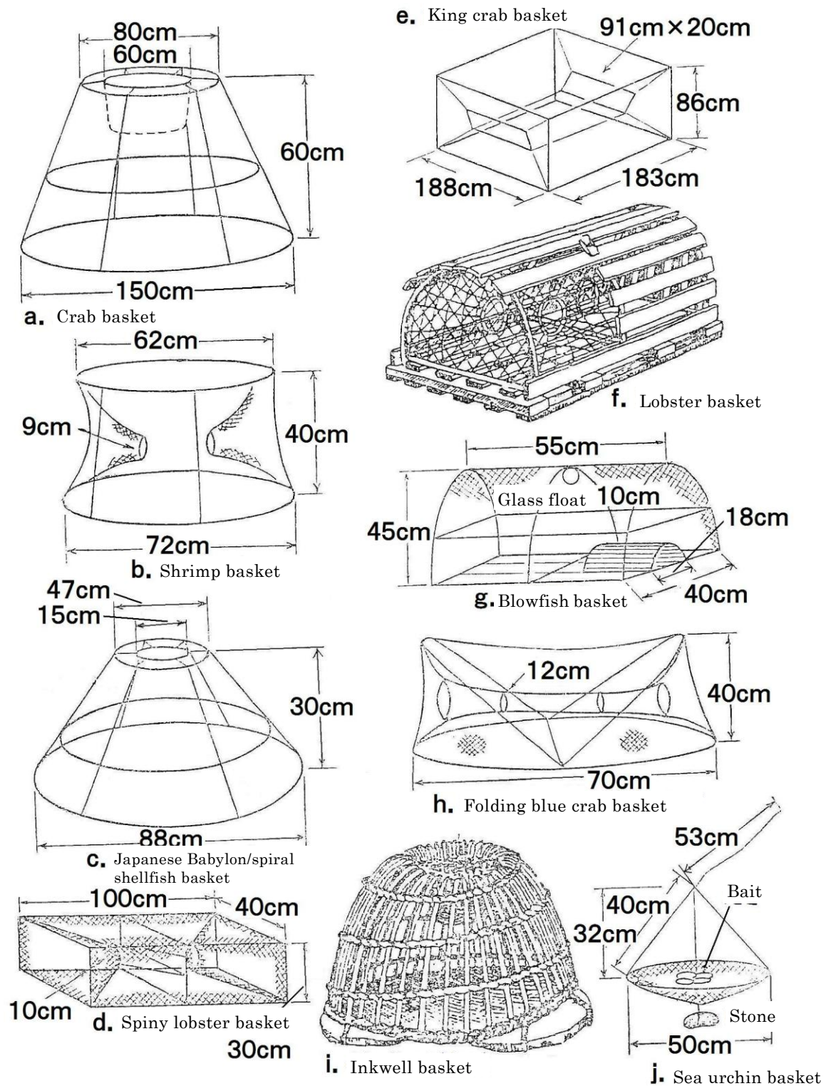
Figure 33: Various basket shapes
