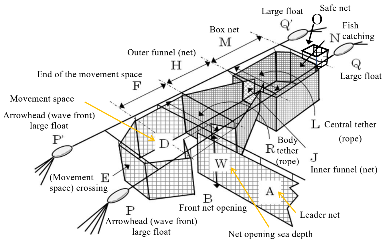
Figure 27: Structure of fixed net and name for each part
