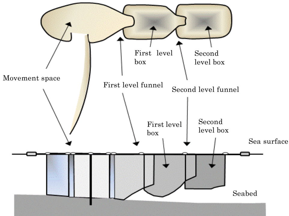
Figure 29: Fixed net with dual box structure (horizontal projection and cross-sectional view)
