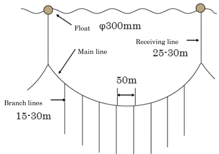
Figure 12: Structure of fishing equipment
