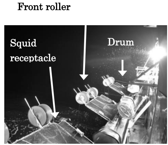
Figure 8: Automatic squid fishing machine in operation
