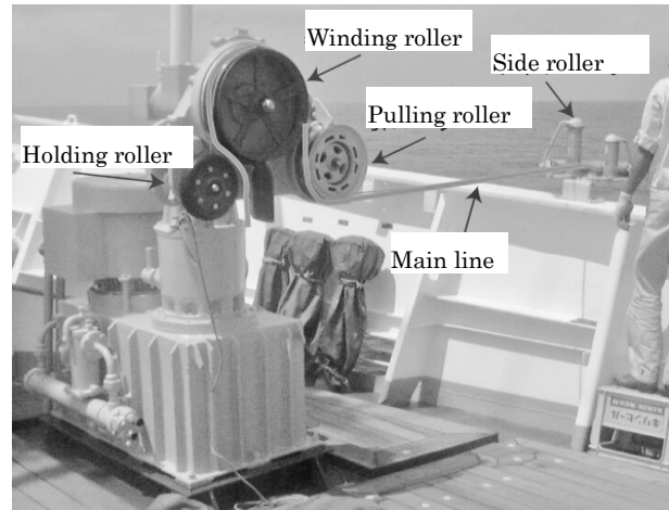
Figure 17: Line hauler
